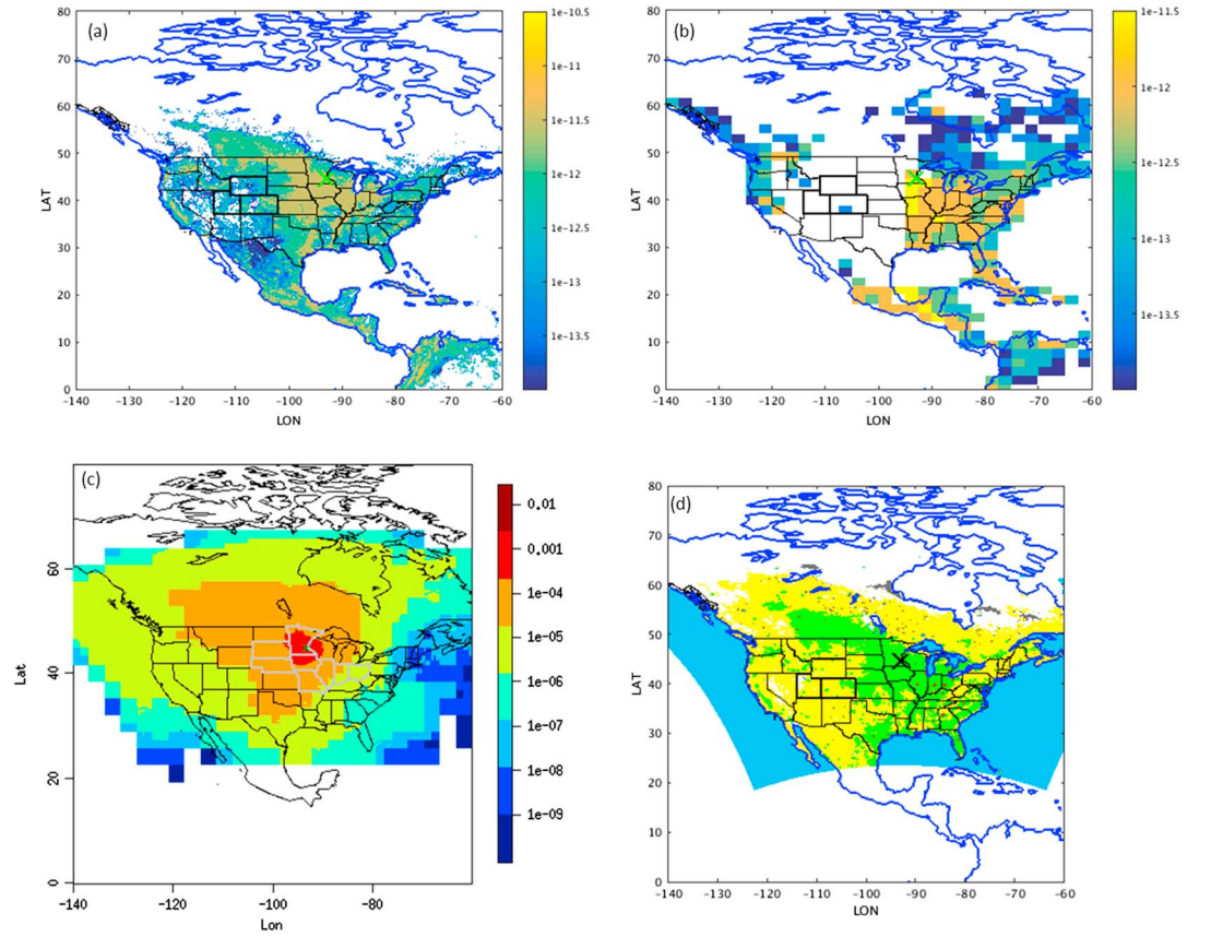
Figure 2. (a) The a priori annual average direct N_2O emissions from agriculture (unit is \log_{10}(\text{kg m}^{-2} \text{s}^{-1}) ); (b) a priori annual average indirect N_2O emissions from agriculture (the coastlines are denoted by blue lines, and the US States are denoted by black lines); (c) annual average source footprint of the tall tower (units are \log_{10}(\text{ppm } \mu\text{mol}^{-1} \text{m}^2 \text{s}) ); the U.S. Corn Belt is denoted by gray lines; (d) land use distribution from U.S. Geological Survey (red, green, yellow, gray, and light blue colors denote the urban, agricultural soils, natural soils, wetlands, and water bodies, respectively).
